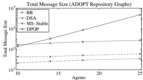
Figure 5: Total size of messages exchanged by algorithms on the ADOPT repository graphs.
