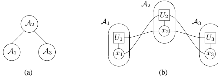
Figure 2: Diagram showing (a) the interactions of agents, \mathcal{A}_1 , \mathcal{A}_2 and \mathcal{A}_3 , and (b) the resulting cyclic factor graph.
