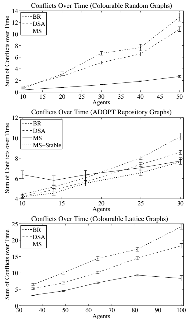
Figure 4: Results for the three graph colouring datasets showing the number of conflicts summed over execution time. Simulation results are averaged over 10 runs on each graph instance, and error bars represent the standard error of the mean.
