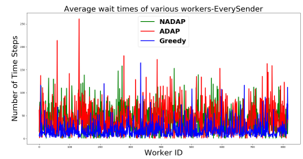
Figure 6: Average waiting times for workers, EverySender dataset
