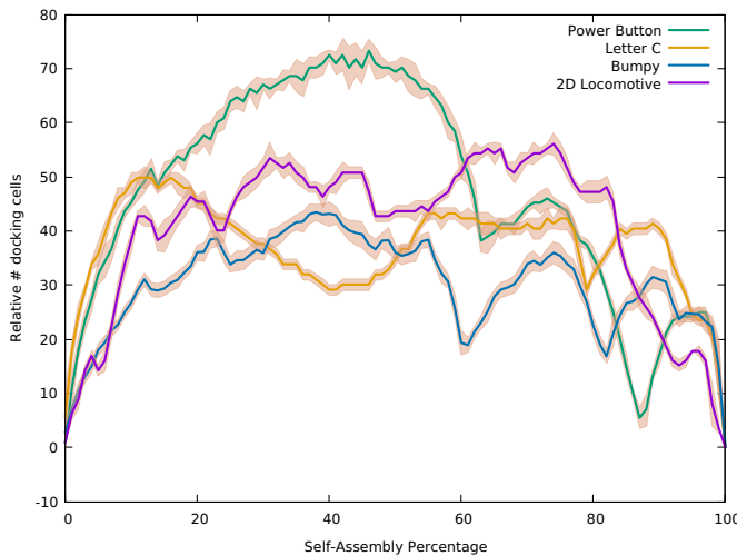
Figure 11: Relative number of available docking positions over the percentage of construction. It shows parallelism of the method by having as many docking positions as possible at the same time. The thick lines represent the standard deviation in a certain construction percentage.
