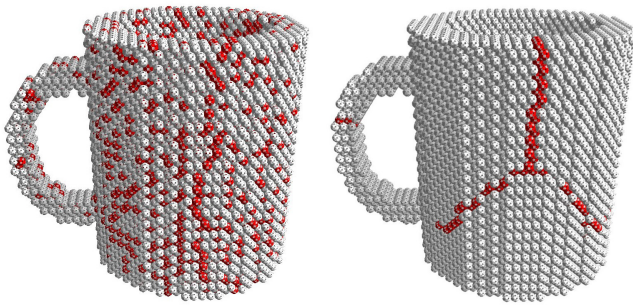
Figure 3: Importance of sequence planning shown on a Mug model made by 12,000 modules. Red modules represent docking problems using two simple planning algorithms. On the left, choosing a stochastic order produces 3,691 modules that does not verify the docking rule. On the right, filling regularly each module neighborhood in sequence results in 231 positions that could not be filled.
