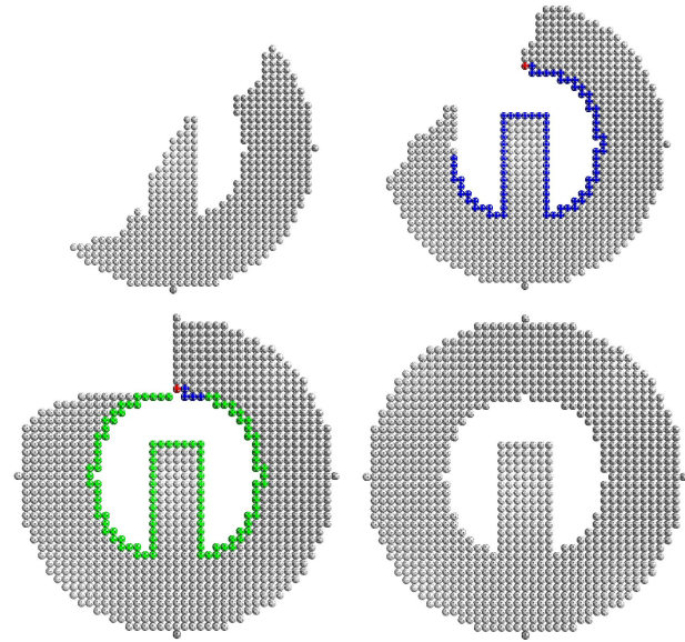
Figure 7: Example of constructing a model with internal hole in a two-dimensional square lattice. The task is parallelized as many positions can be filled at the same time. The modular robot drawn in red detects a section of line merge made by the internal hole. It sends a message following the inner border (blue modules) and waits for an unlock message. At the moment the message arrives in the south-west position of the red module, the module sends a response in the reverse path (green). This verification is necessary before a module docks on the red module west side in order to have no position blocked.
