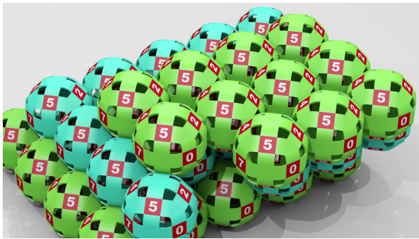
Figure 2: Catoms in FCC lattice which admit modules to have up to 12 connected neighbors.
