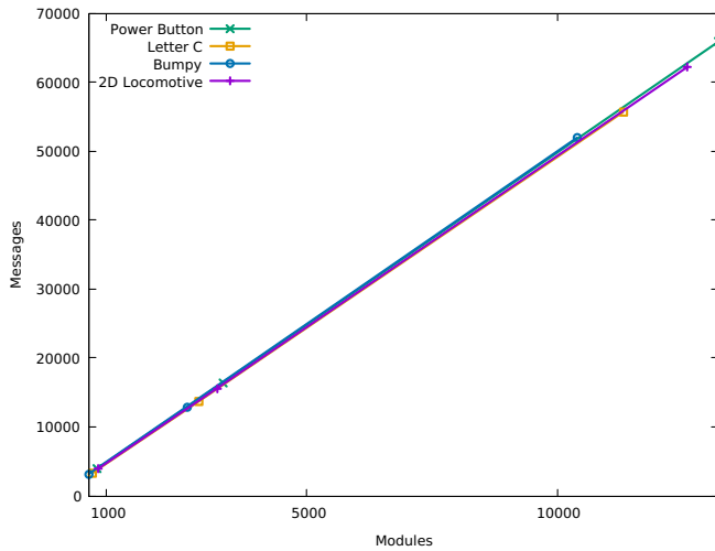
Figure 10: Number of messages for four topologically different representations on three different scales. The number of messages remains linear and similar across all representations.
