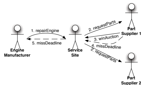
Figure 5: Original scenario representation.
