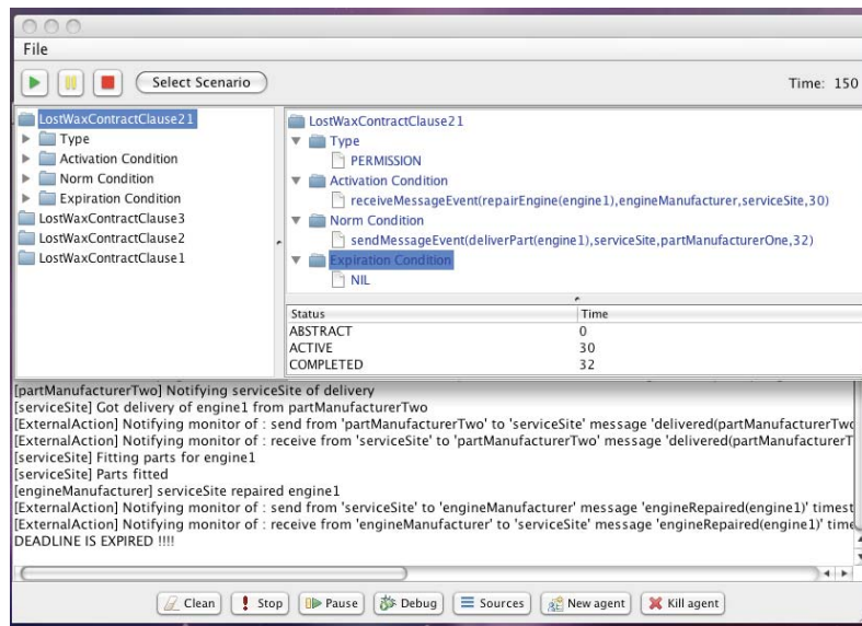
Figure 4: Screenshot of the monitoring application.
