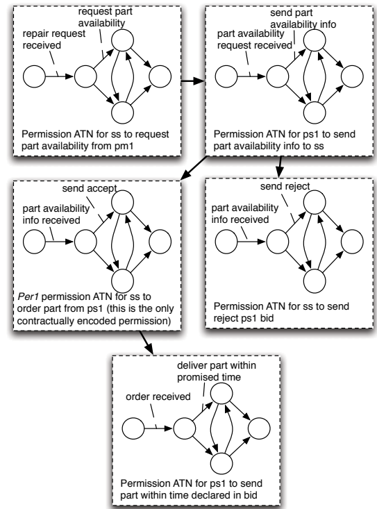
Figure 6: Chained explanation ATNs for Scenario 1
