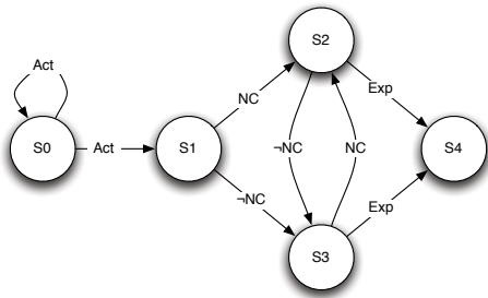
Figure 2: The ATN used to represent norms.
