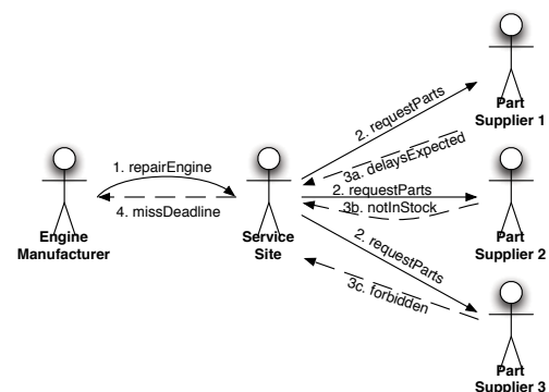
Figure 8: Original scenario leading to failure.
