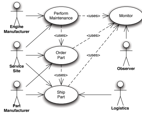
Figure 1: Use cases and interactions (in UML).
