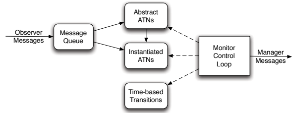
Figure 3: Overview of the monitor control loop.
