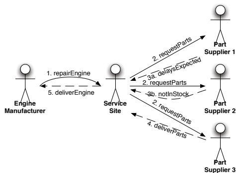
Figure 9: Relaxed restrictions lead to success.
