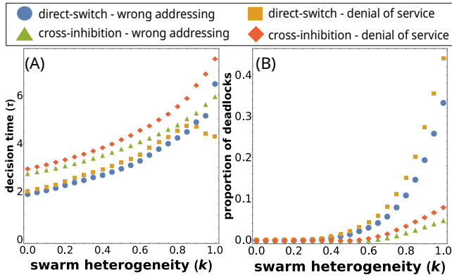
Figure 5: (A) Decision time \tau computed as the amount of time to reach the decision threshold \theta = 0.7 for either option. (B) The proportion of conditions in the parameter space ( q, z_B ) where the swarm remains deadlocked at indecision ( (A(t_{MAX}) < \theta) \wedge (B(t_{MAX}) < \theta) ), i.e., the proportion of the yellow area of Fig. 1. In both panels, we report results for both models, both attacks, and various values of the swarm composition k \in [0, 1] .
