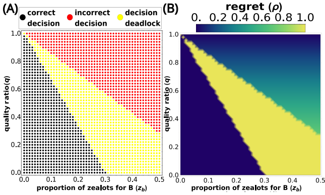
Figure 1: Representative results of the homogeneous swarms composed of agents using the direct-switch and voter rule (system (6) with k = 1 ) under wrong-addressing attack in the parameter space (q, z_b) . In (A), the three colours show the decision outcome for each (q, z_b) : the black points represent convergence of the group opinions to option A ( A(t_{MAX}) \geq \theta ), the red points represent group convergence of the opinions to option B ( B(t_{MAX}) \geq \theta ) and the yellow points represent a decision deadlock ( (A(t_{MAX}) < \theta) \wedge (B(t_{MAX}) < \theta) ). In (B), we use the decision outcome to compute the regret \rho which we represent as a colour map, where decision deadlocks lead to the highest regret (yellow region with \rho = 1 ), and accurate decisions to the zero regret (dark blue region with \rho = 0 ).
