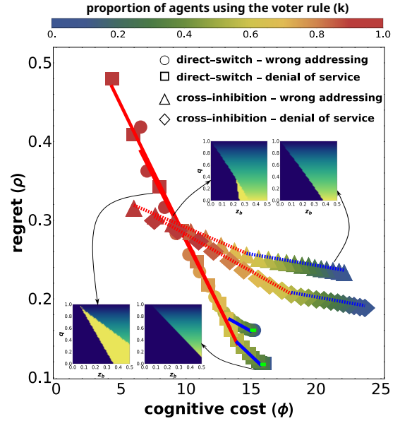
Figure 3: Cost-performance trade-off as the relationship between the regret \rho and the cognitive cost \phi in making the decision, for both models, direct-switch of Eq. (6) and cross-inhibition of Eq. (7), and for both types of attacks, denial-of-service ( z_a = 0.05 ) and wrong-addressing ( z_a = 0 ). Each point represents the average regret (y-axis) computed across all tested values of parameters q and z_b ; in other words, we report the average value of the colour maps of Fig. 1B for each k \in [0, 1] . Each point’s k value is colour-coded according to the top bar. The insets show the parameter space (q, z_b) computed for some specific k values, which when averaged gives the regret of the plotted point k (the colour maps for all tested conditions are available in the supplementary material [1]). We can observe that the resulting lines in the cost-performance space can be approximated well through piecewise linear functions (lines overlaid onto the data points, see Table 1).
