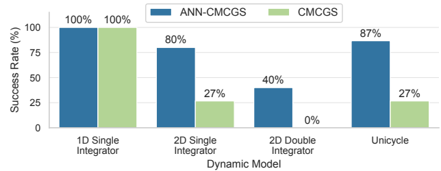
Figure 2: Success rates at fixed node sampling budgets for ANN-CMCGS (ours) and CMCGS.
