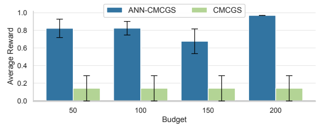
Figure 3: Performance of ANN-CMCGS (ours) and CMCGS with unicycle dynamics across increasing node expansion budgets. Results averaged over 20 episodes; error bars show standard error of mean.
